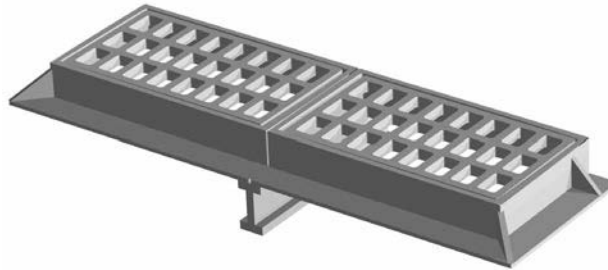
Illustrating V-4243Z1 left and right hand frames with I-beam and two grates
